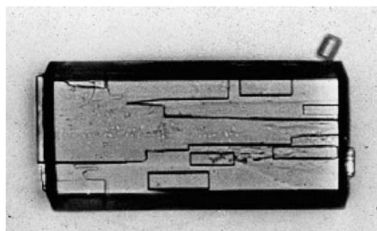
Figure 4. Uric acid phase II epitaxially grown on phase I.
