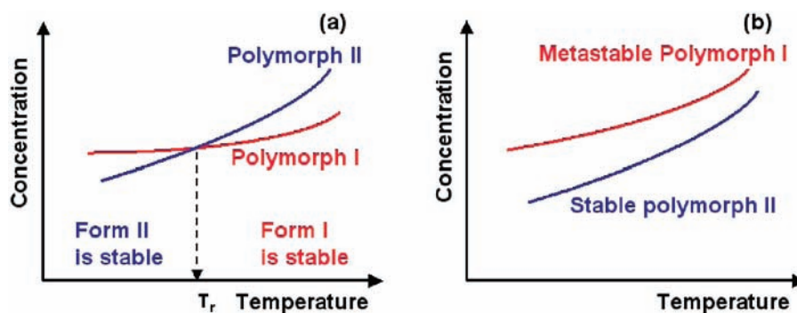
Figure 2. Solubility curves for two polymorphs I and II, related either enantiotropically (a) or monotropically (b).
