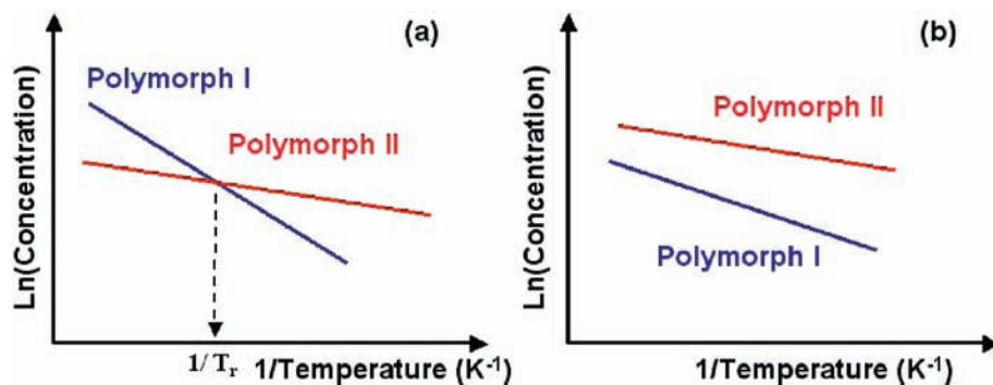
Figure 3. van't Hoff plot of solubility for a dimorphic system related either enantiotropically (a) or monotropically (b).
