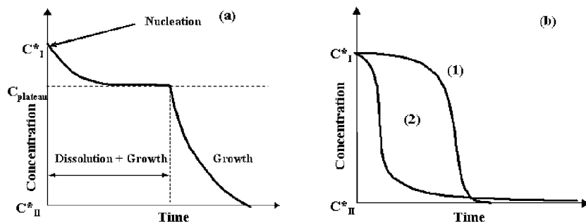
Figure 6. Concentration vs time during a polymorphic transition in solution, C^*_I and C^*_{II} are the solubilities of the two phases, (a) general profile and (b) limit profiles; curve (1) transformation is controlled by growth of the stable form (II) and curve (2) transformation is controlled by dissolution of the metastable form (I).
